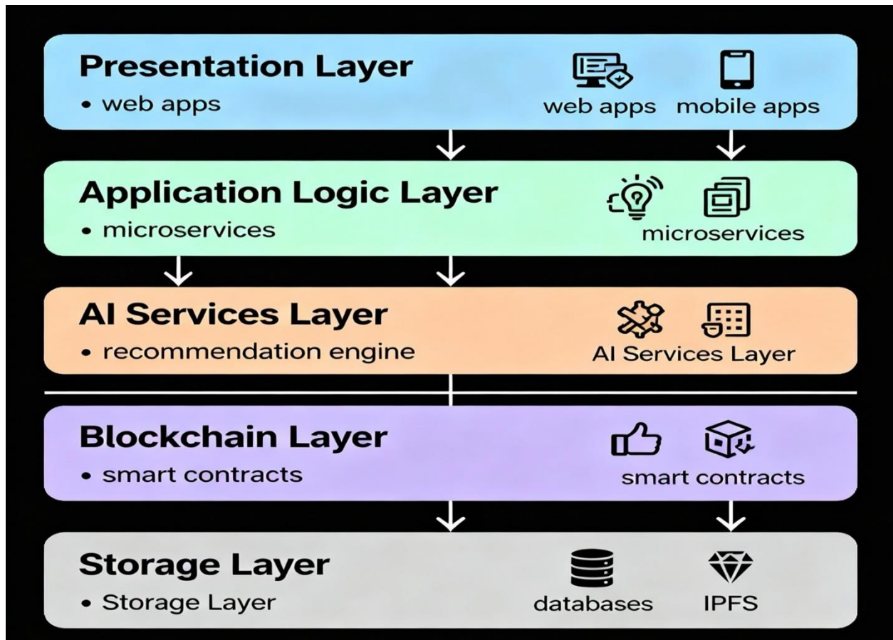
Figure 2: Architecture overview
